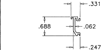
⑥ GLAZING ADAPTER
