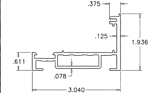
①A FLUSH FRAME HEAD/SILL/JAMB
