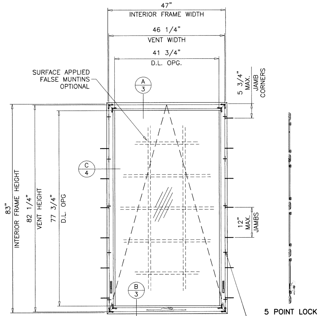
TYPICAL ELEVATIONS TESTED UNITS
